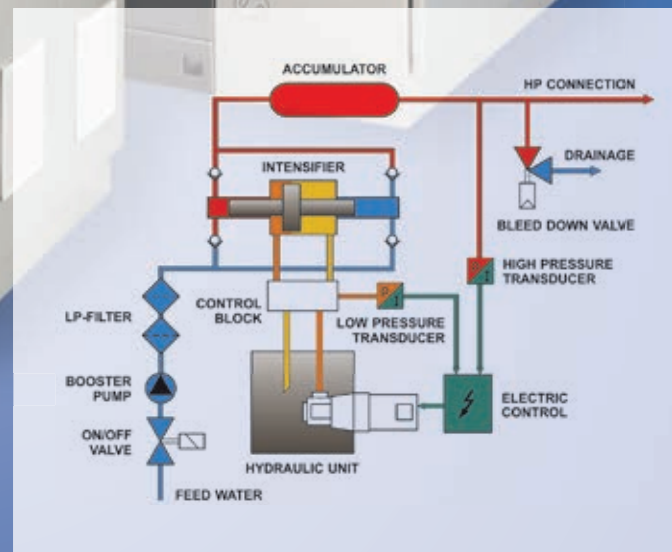
System diagram for high pressure pump SERVOTRON®
